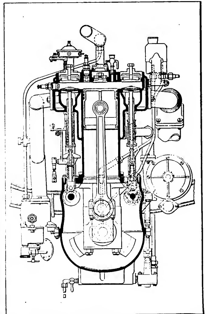
Fig. 12—Transverse section through the front cylinder of a Pierce-Arrow six-cylinder motor
